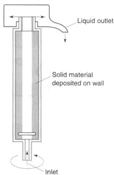
Fig. 22.8 Tubular-bowl centrifuge.
