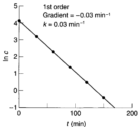
Fig. 7.1 First order.
