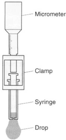
Fig. 5.6 Drop volume or drop weight method.
