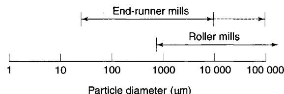
Fig. 11.7 Size reduction range for compression methods.
